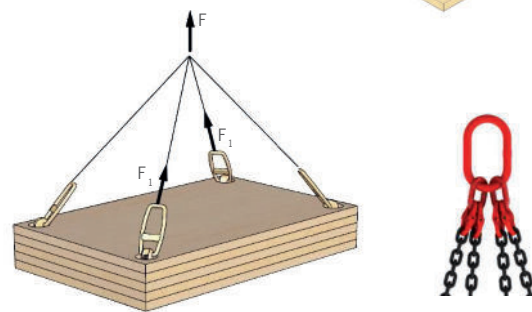
statically indeterminate hanger www.wuerth.de | www.pewag.at
