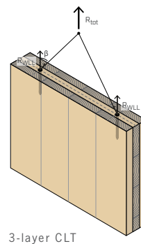
3-layer CLT
