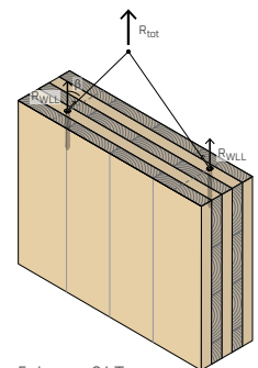
5-layer CLT
