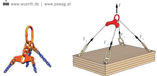
statically determinate hanger with compensating seesaw www.pewag.at | www.wuerth.de
