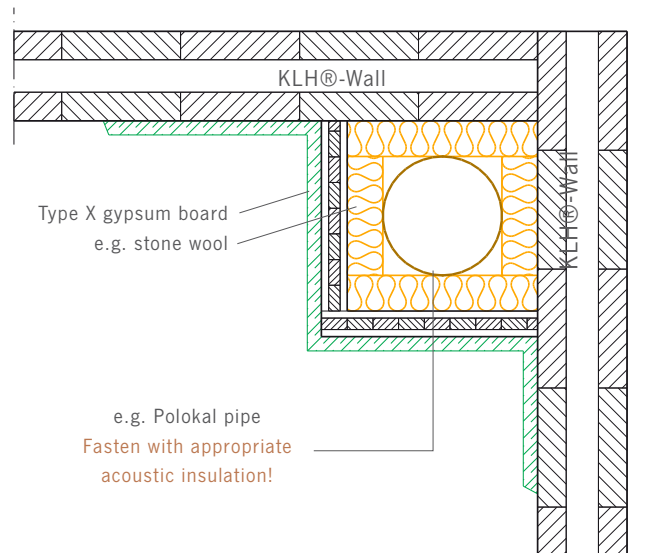
Fig. 55 – Schematic diagram – downpipe in installation shaft – ground plan
