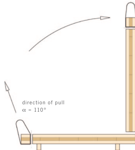
Load securing in accordance with legal regulations and provisions
